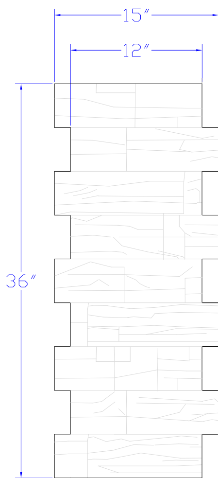
Showing 1 Of The 4 Panels Needed For One Full Column
